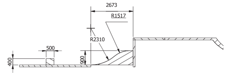
Section F - F
