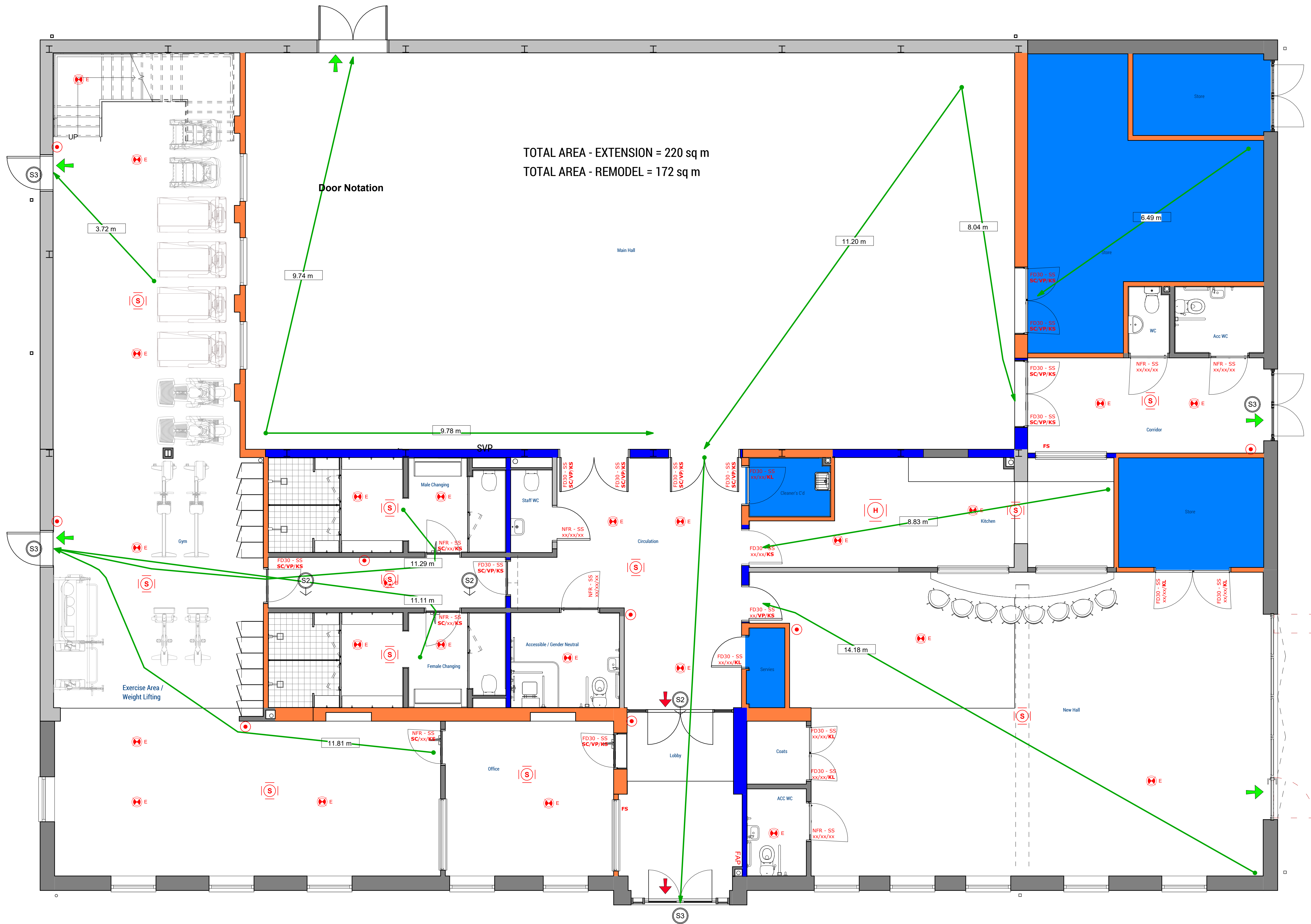
Ground Floor - Fire Strategy 1 : 50
