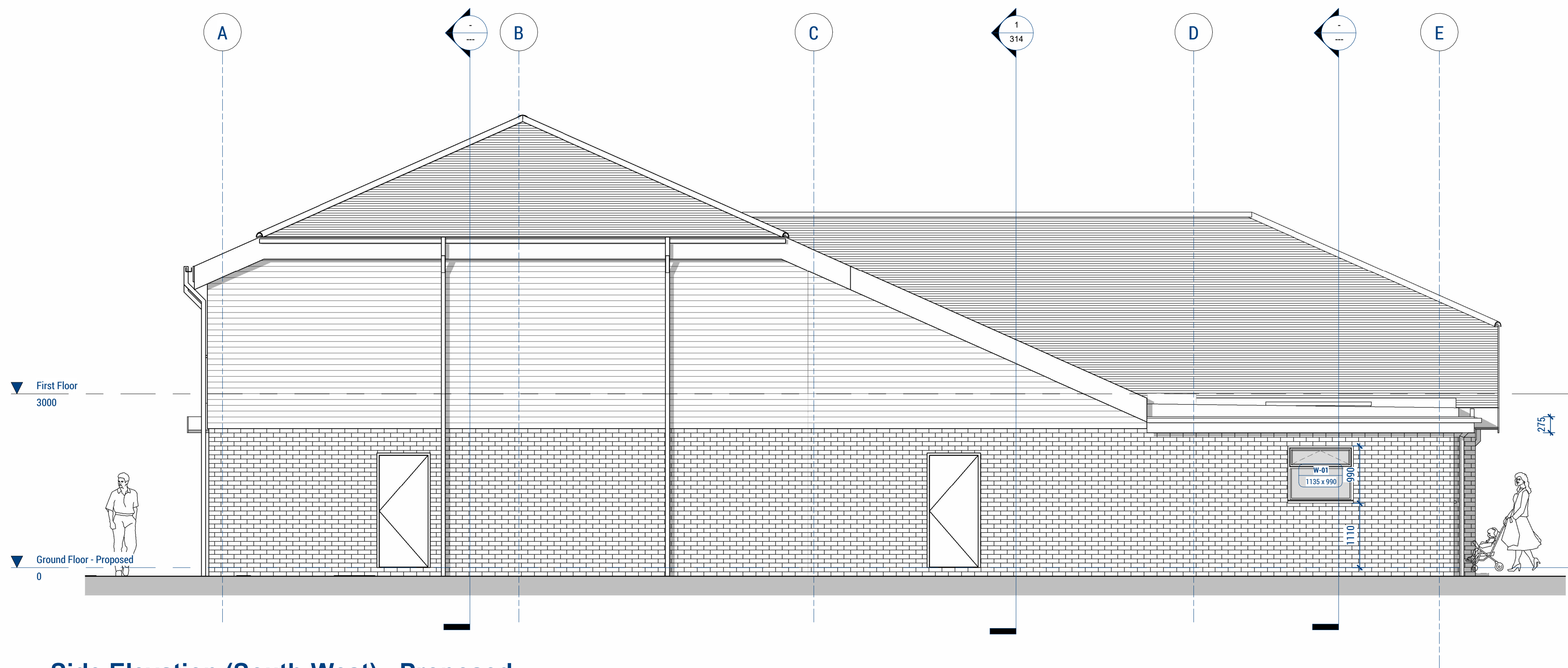
Side Elevation (South-West) - Proposed 1 : 50
