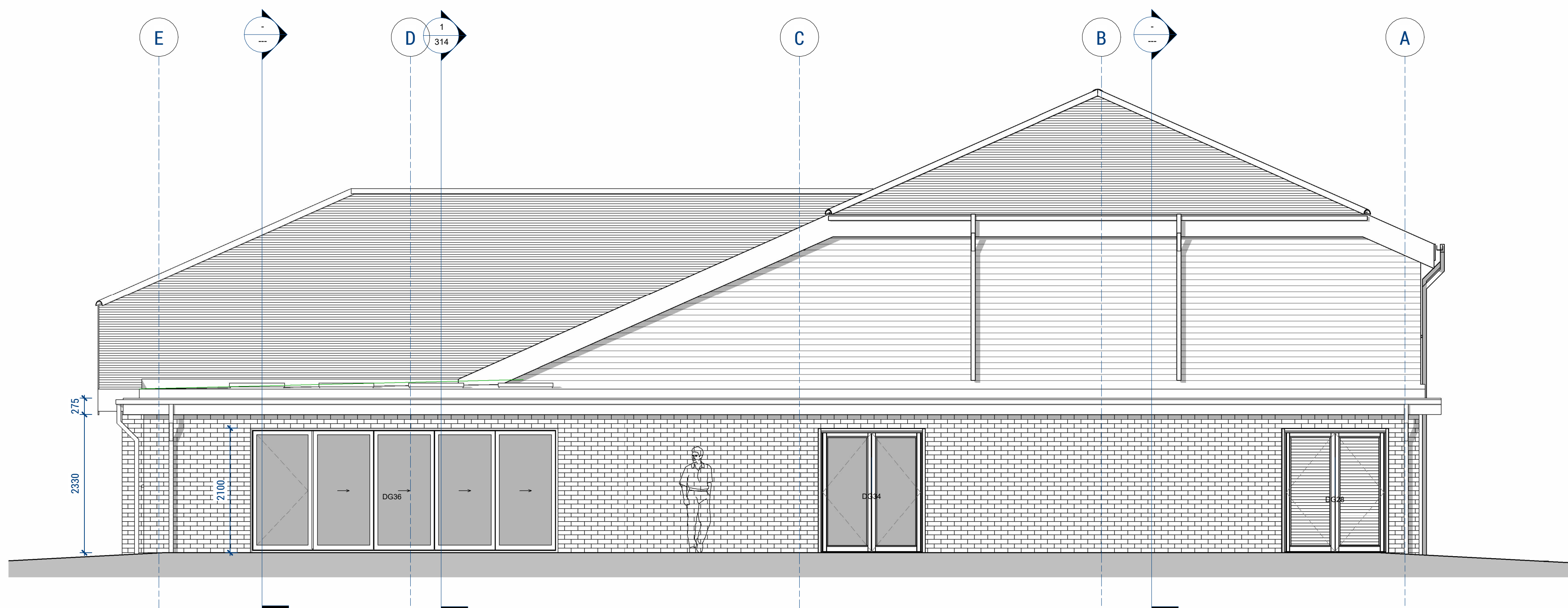
Side (North-East) Elevation - Proposed 1 : 50
