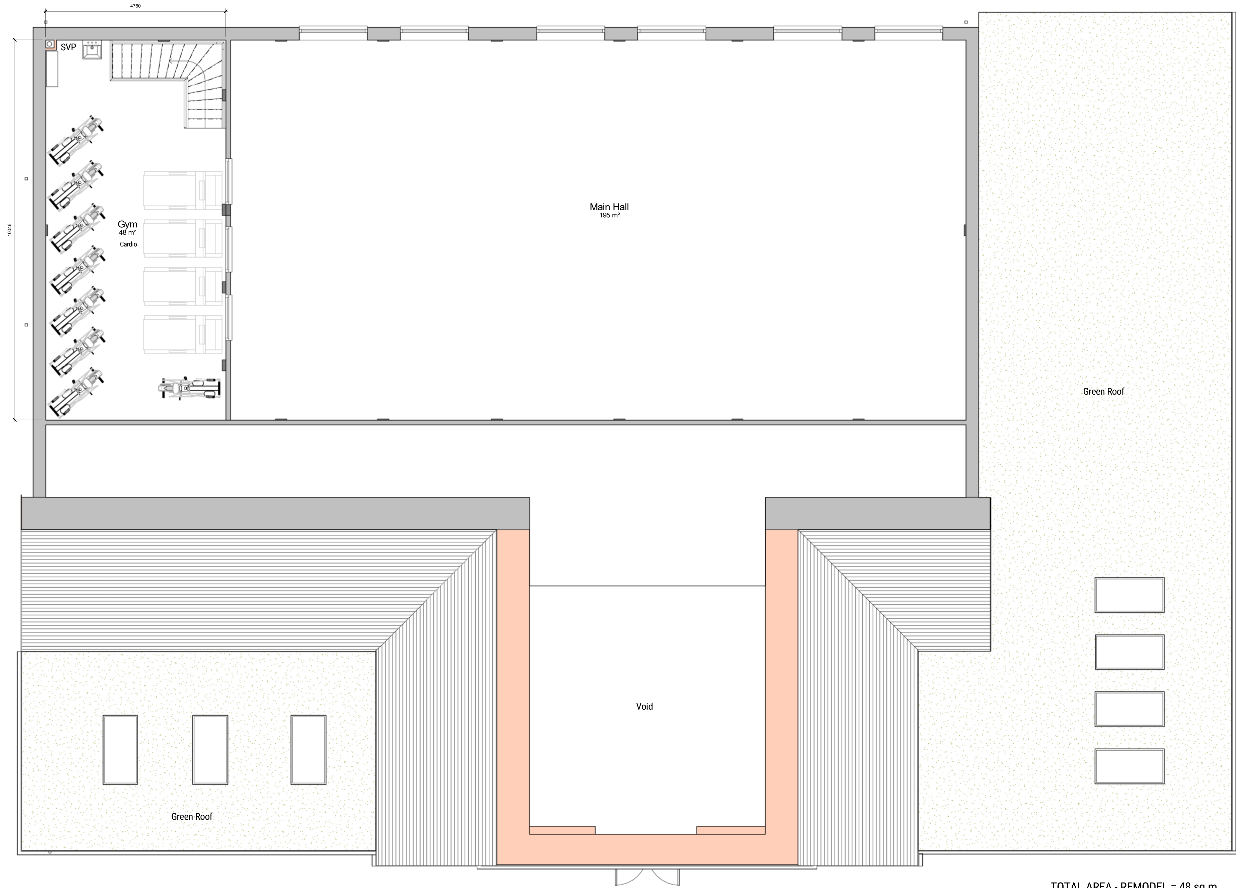
First Floor - Proposed 1 : 50
