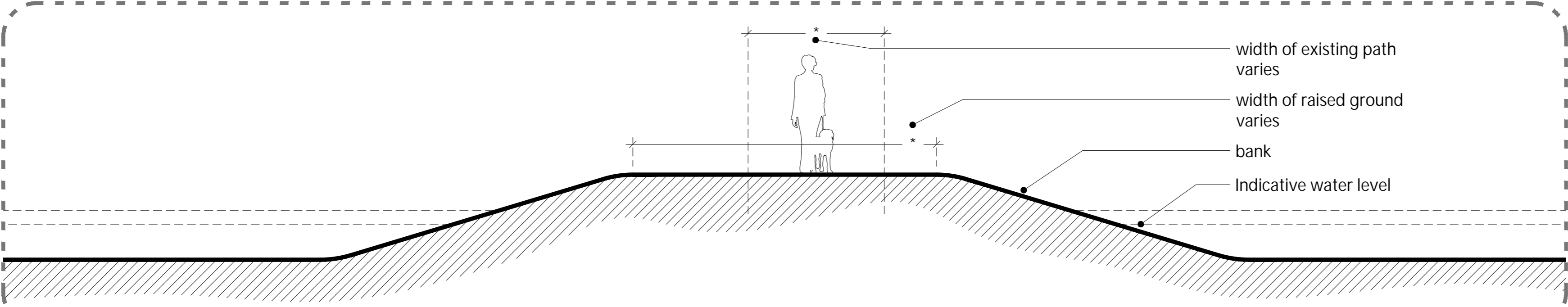
Section A: Existing Path (1:50)
