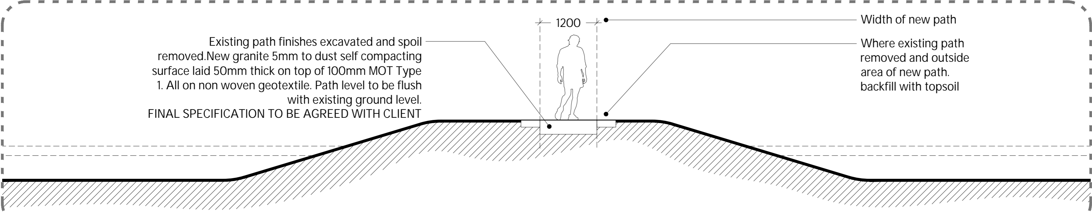
Section B: Proposed Path (1:50)
