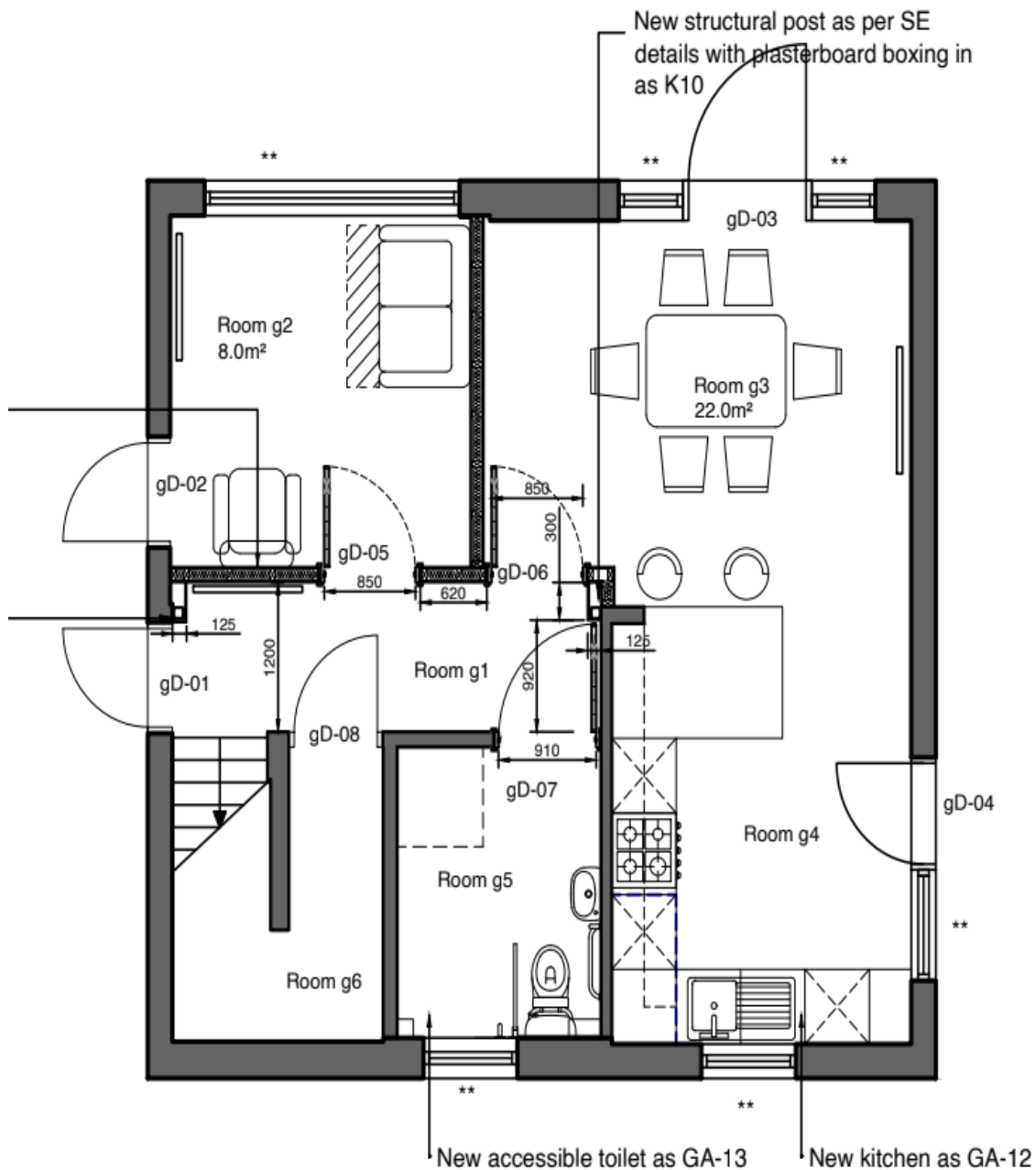
A | PROPOSED GROUND FLOOR PLAN GA-10 | 1:100@A3
