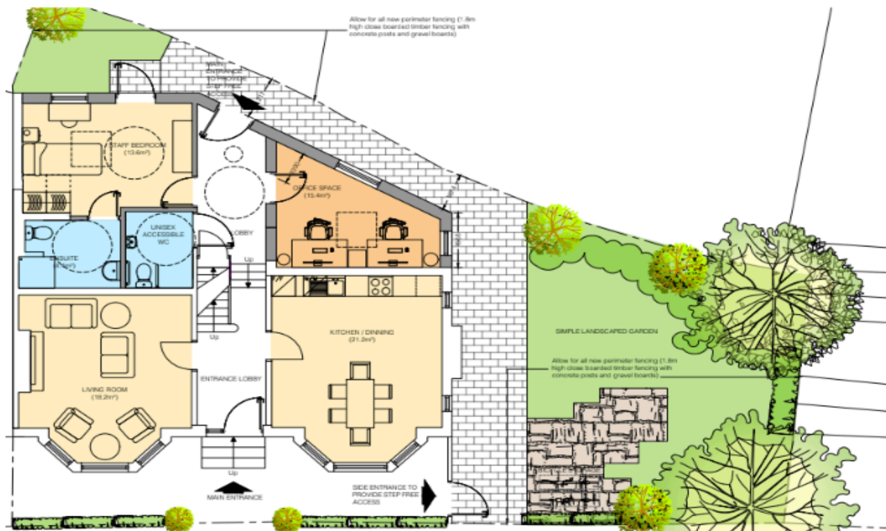
PROPOSED GROUND FLOOR PLAN SCALE 1:50 @ A1
