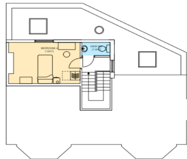
PROPOSED SECOND FLOOR PLAN SCALE 1:50 @ A1
