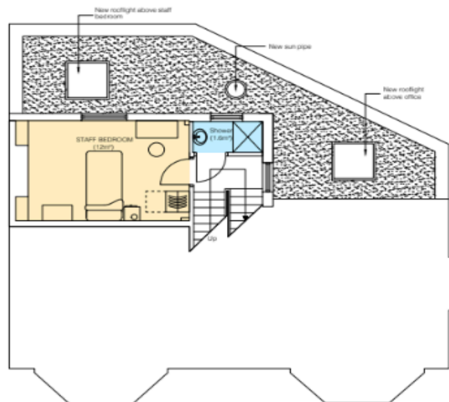
PROPOSED GROUND FLOOR MEZZANINE PLAN SCALE 1:50 @ A1
