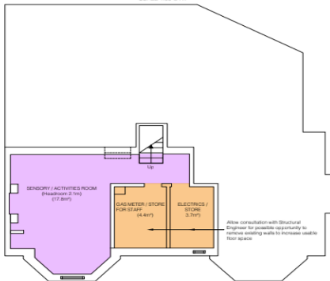
PROPOSED GROUND FLOOR PLAN SCALE 1:50 @ A1
