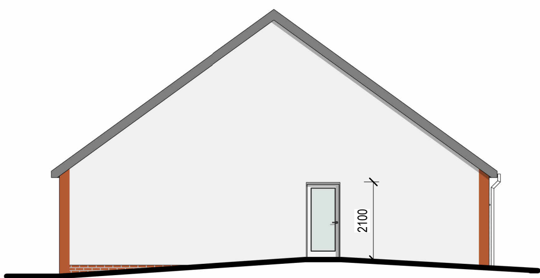
West Elevation (Existing) 1 : 100
