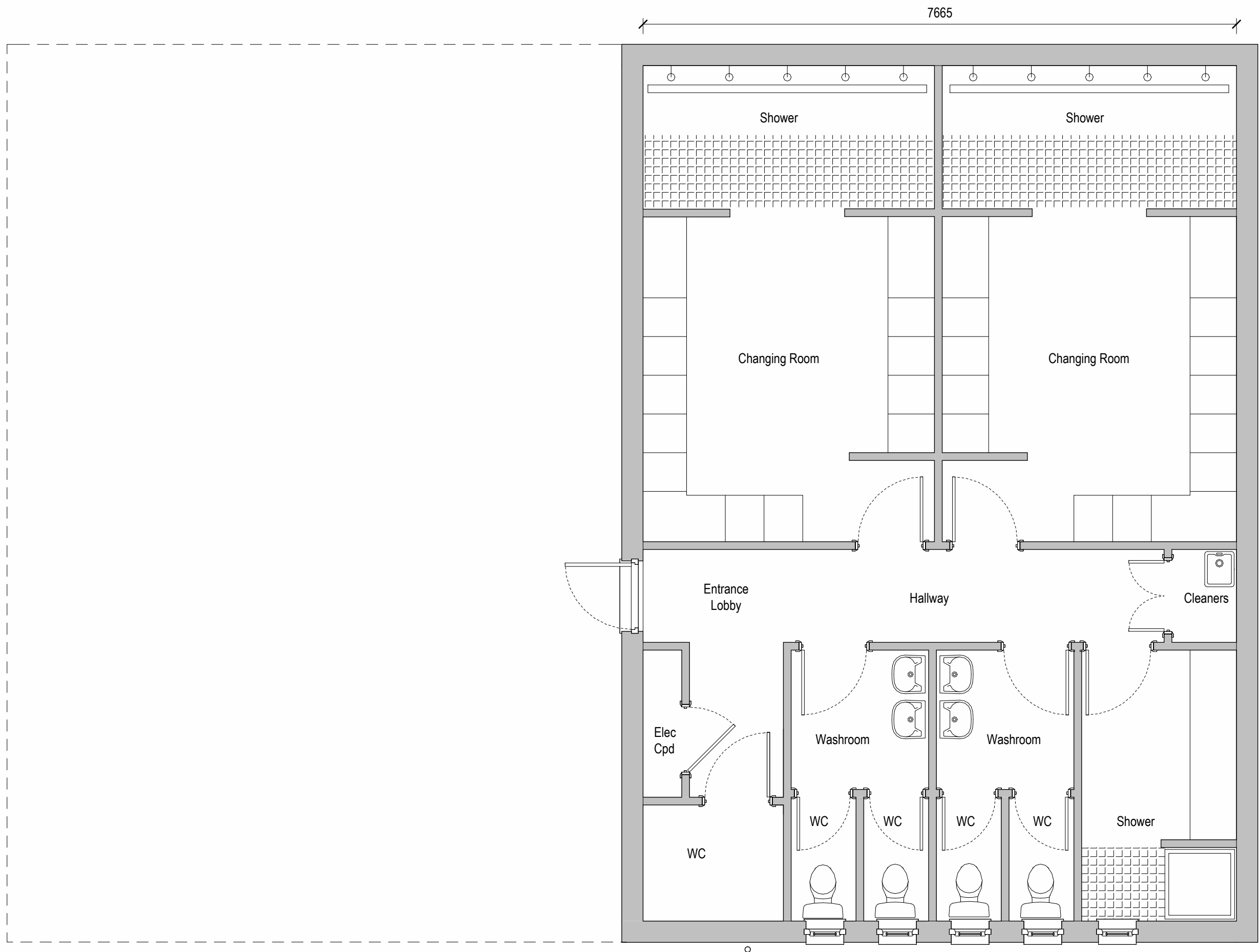
Existing Ground Floor 1 : 50
