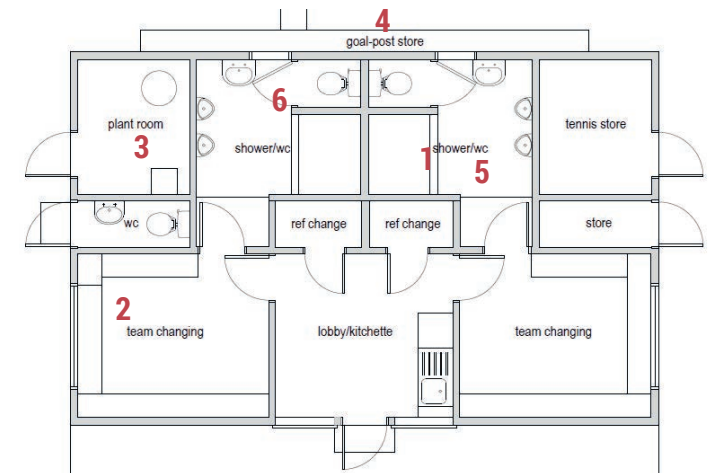
5. SHOWER / WC
