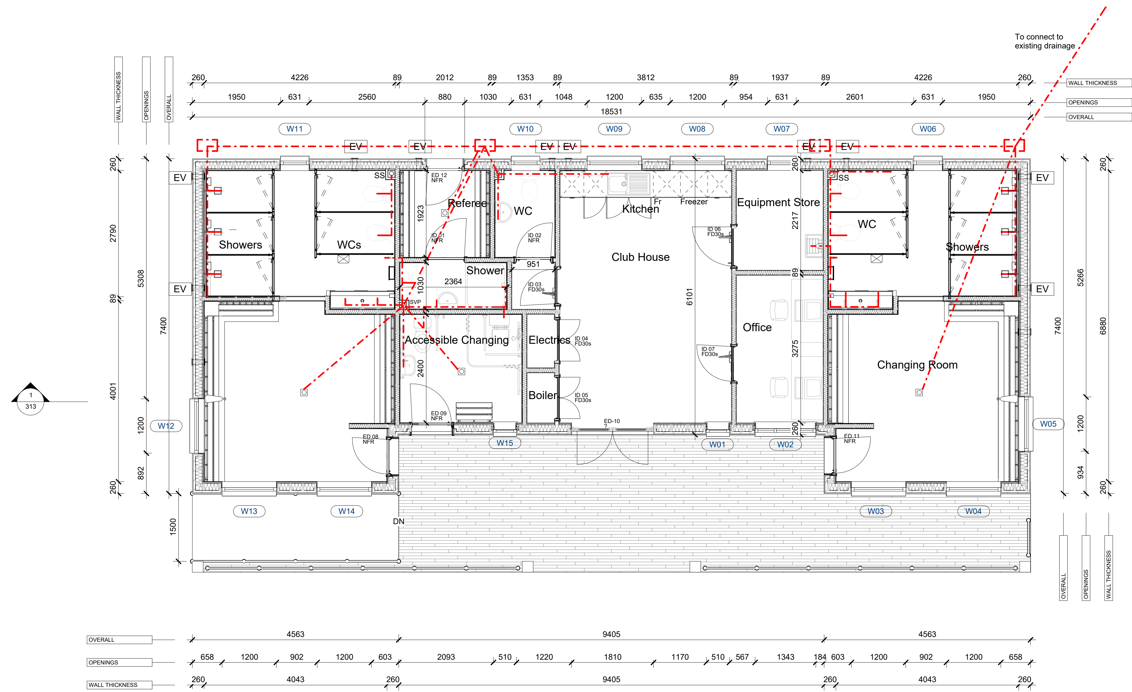
Ground Floor as proposed 1 : 50
