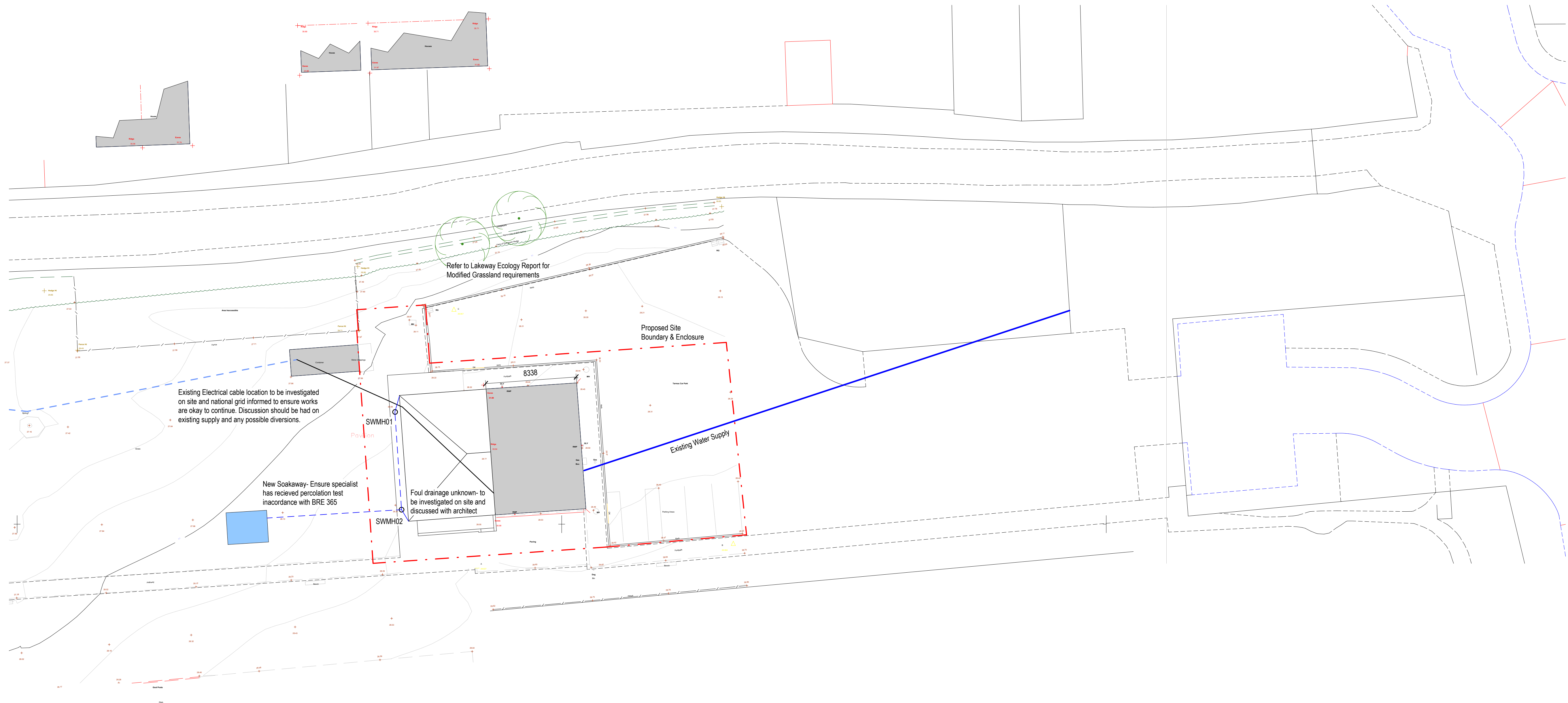
00 Proposed Site Plan 1 : 200
