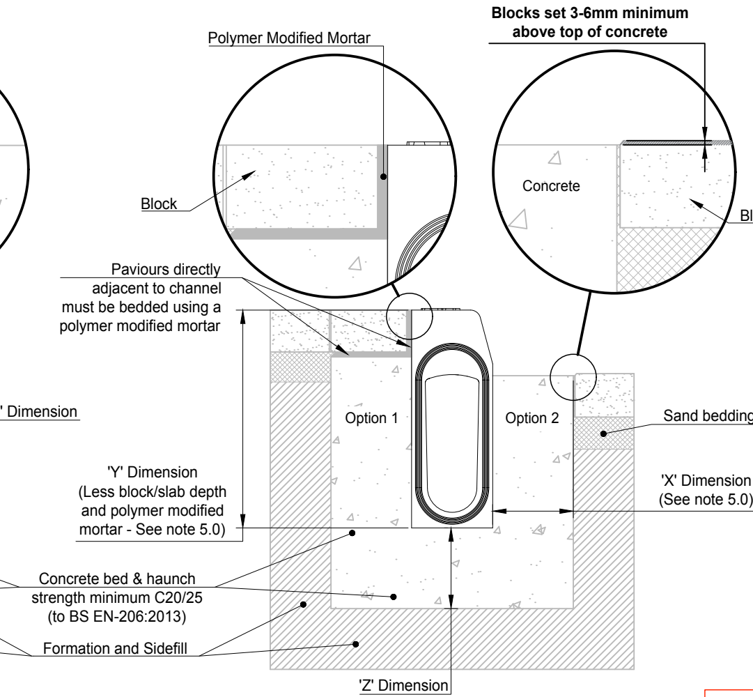
1 : 10 ACO KerbDrain KDHB Block Pavement (Option 1 and 2)
