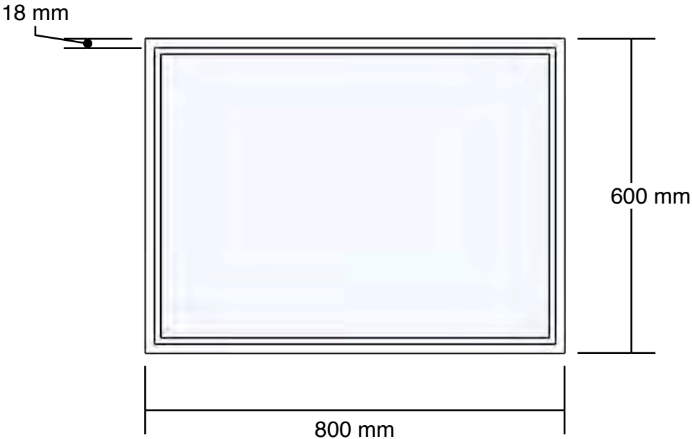
Plan 1:10 @ A3 PAGE 10
